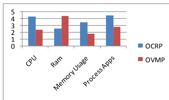
Figure 4. Performance results of Comparison with OCRP & OVMP
