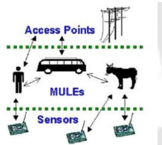
Figure 3. The three tiers of the MULE architecture
