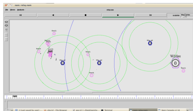
Figure: Nam output for VHO-with ad-hoc type
